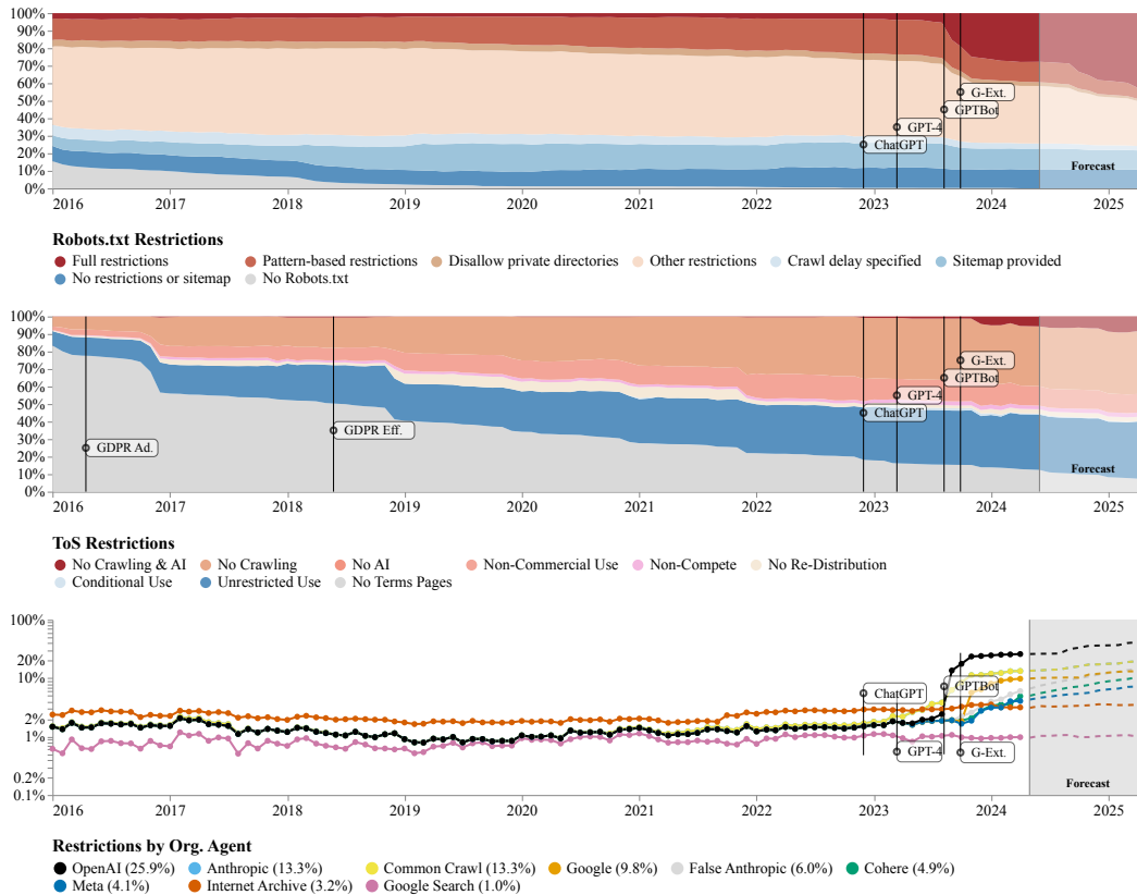
Figure 1: A temporal analysis, from 2016 to April 2024, of the web consent signals in HEAD C4 , a sample of the largest and most critical web domains. The colored regions represent the restriction categories as a portion of the total tokens in HEAD C4 . We also use SARIMA methods to forecast trends a year into the future. Top: Ascending categories of robots.txt restrictions for the AI Organizations: Google, OpenAI, Anthropic, Cohere, Meta, Common Crawl, and the Internet Archive. Middle: Ascending categories of Terms of Service restrictions (taxonomies described in Table 2). Bottom: A breakdown of robots.txt restrictions by organization—the April 2024 restriction rates are listed in the legend.
