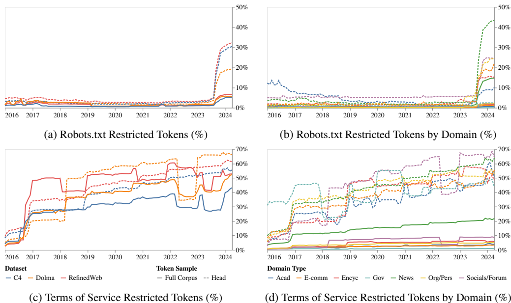
Figure 2: A temporal depiction of the percentage of restricted tokens across both the Full Corpus and the HEAD_{All} sample—the largest and most critical data sources. The robots.txt analysis (top) and Terms of Service analysis (bottom), are each broken down by corpora—C4, RefinedWeb, and Dolma (left),—and by the restrictions by domain type, averaged across corpora (right).
